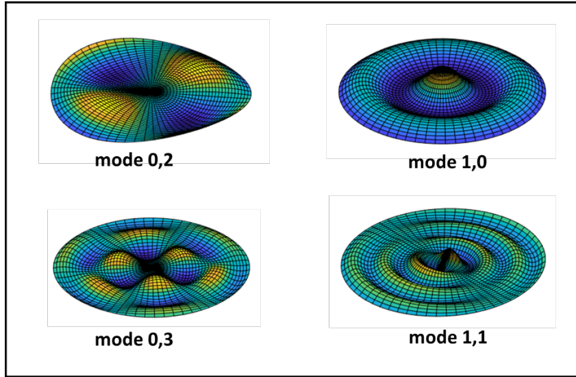
Figure 7: The first four vibrational modes of a free edge disk.
